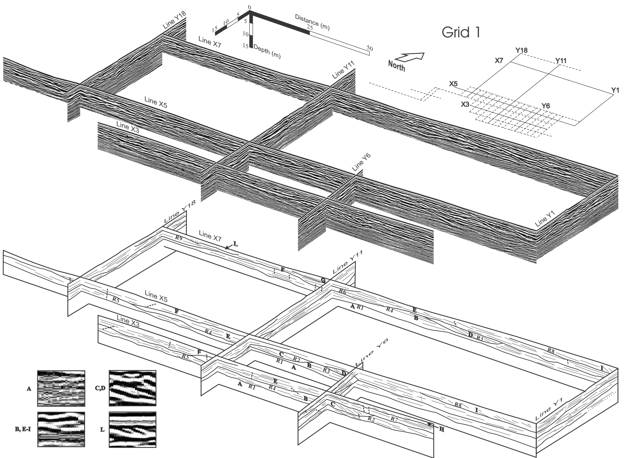
Fig. S1. Processed and interpreted fence diagrams for selected lines of pseudo-3D grid 1 (Figs. 1 and 2B and C) on Young Lake esker-like ridge. Hairlines show interpreted and generalized interior reflections between bounding surfaces (bolder lines). The relative location of these selected profiles are represented by the solid lines on the grid map (top right). Example thumbnail images of radar reflections for each radar element are presented at the bottom left (refer to text for detailed descriptions). Dashed lines demarcate offset reflections. GPR profiles are shown with no vertical exaggeration.
