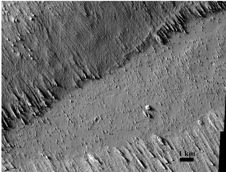
Fig. 4. Portion of THEMIS image V13163010, showing a random network of wispy SRs (Area04, Table 1; located near 2.1^{\circ} N 153.8^{\circ} E). The NW-SE-oriented lemniscate forms at upper left and lower right are inferred yardangs. A sinuous trough of unknown origin is visible near image center. North is up and illumination is from the left.
