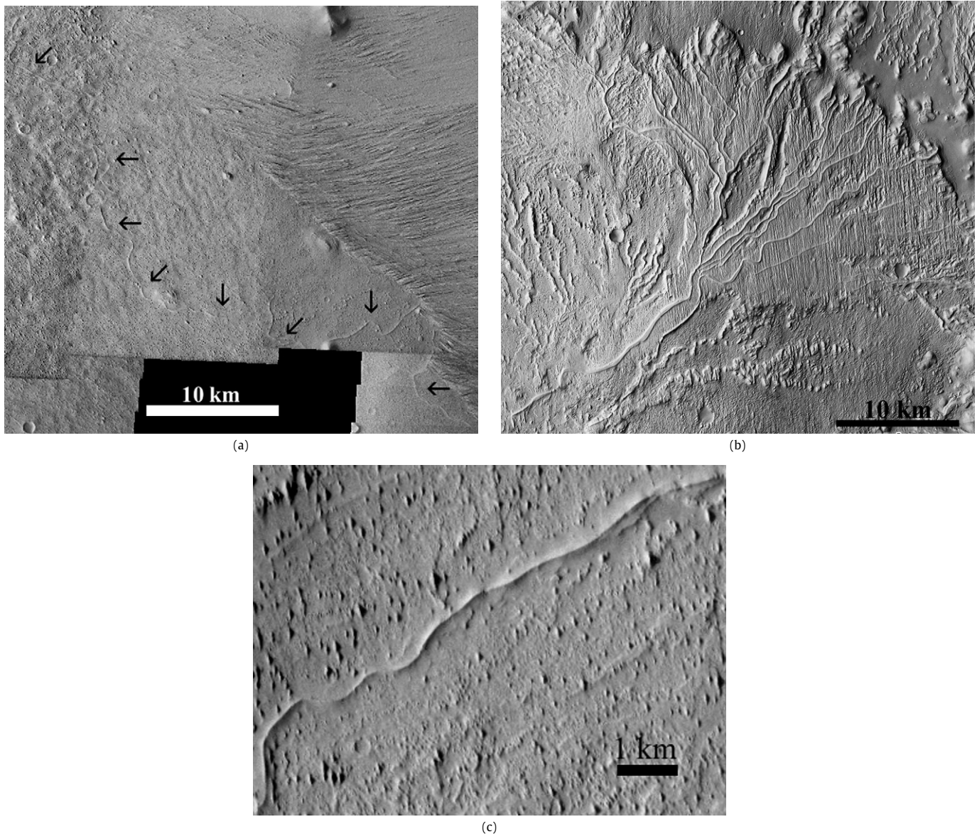
Fig. 2. Examples of thin SRs. On all images, north is up and illumination is from the left. (a) THEMIS image mosaic showing an isolated, thin SR (Area01, Table 1; located near 2.9° S 152.0° E) denoted by the arrows. The sub-parallel lineations at image right are inferred yardangs. (b) CTX mosaic showing a branched network of thin SRs (Area43_C, Table 1; located near 6.2° S 151.6° E). Extensive yardangs are oriented NNW-SSE across image. (c) Portion of THEMIS image V18393002, showing an isolated, thin SR (Area31_C, Table 1; located near 4.8° S 151.3° E) with a sharp medial ridge. The short, lemniscate hills oriented NW to SE throughout the image are inferred yardangs.
