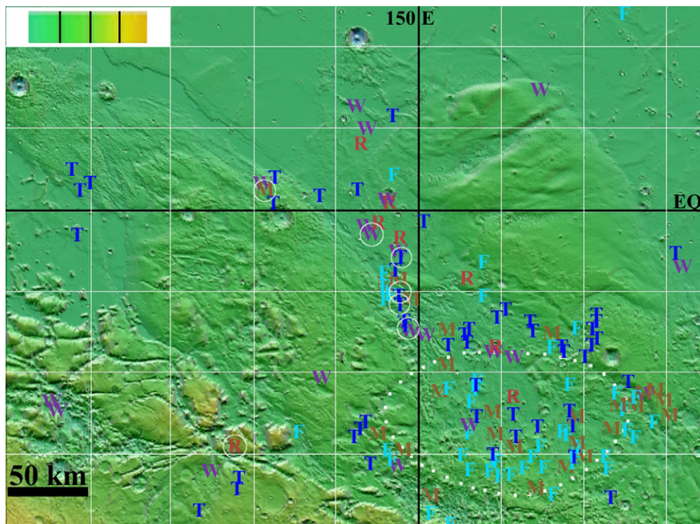
Fig. 9. Shaded relief MOLA topography with illumination from the north overlain by color MOLA topography; color bar denotes elevations from -3000 m (blue) to 1000 m (orange) in 1000 -m increments. Letters indicate individual types of SR: dark blue 'T' indicates thin; light blue 'F' indicates flat; purple 'W' indicates wispy; red 'R' indicates rounded; and brown 'M' indicates multilevel. White circles surround SRs that are connected to fan or delta forms. The black rectangle shows the location of Fig. 14a. The white dots show the location of the broadly circular depression mentioned in Section 3.3.2. The black grid lines are at the equator and 150^\circ E; the white grid lines are every 2 degrees.
