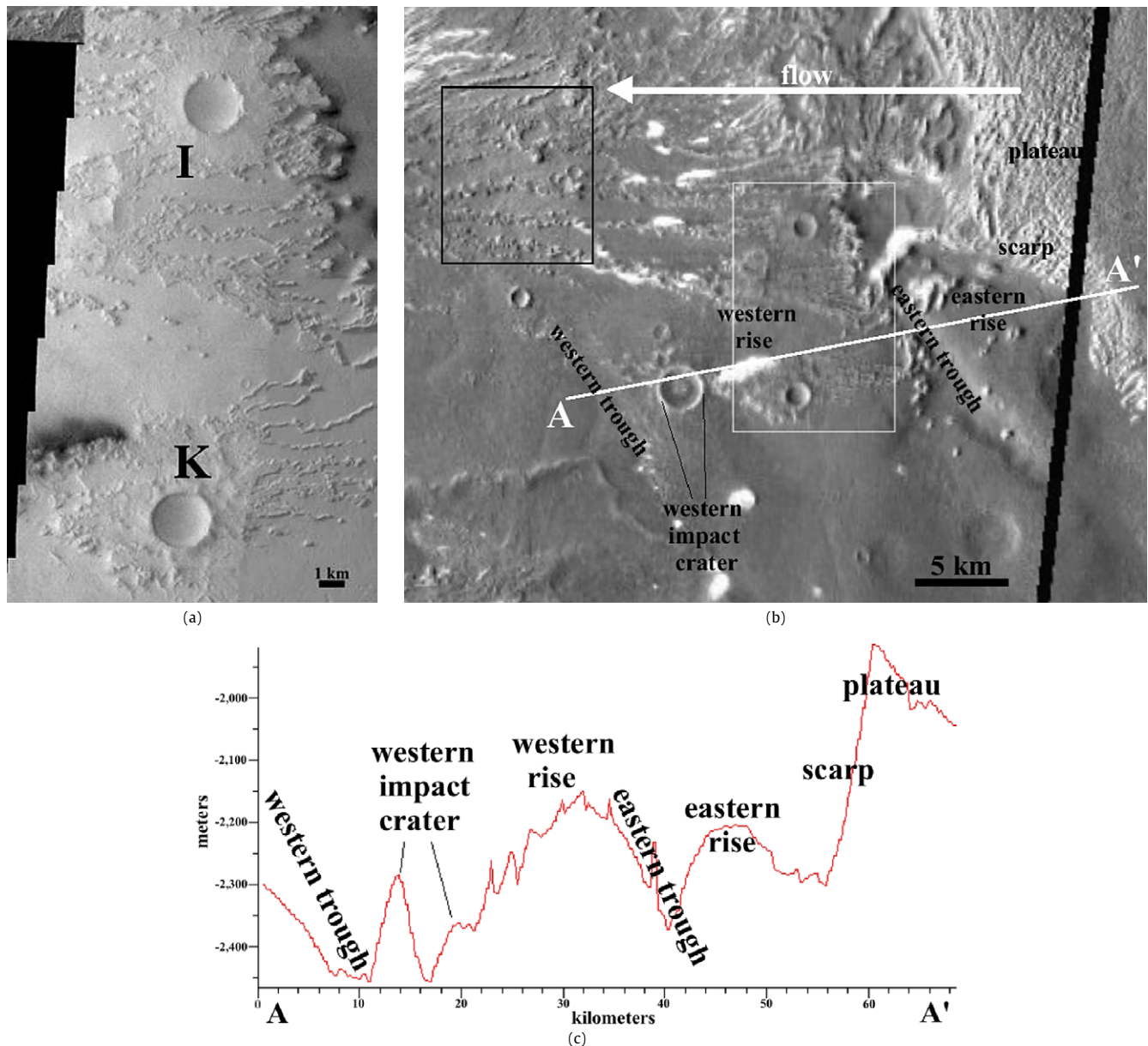
Fig. 7. SRs associated with impact craters. (a) THEMIS visible image mosaic showing two SRs associated with impact craters centered near 5.3^{\circ} S 155.3^{\circ} E. They are classified as sub-parallel based on THEMIS visible mosaics, although the global THEMIS day IR mosaic (b) shows that they connect to the west. 'I' denotes a multilevel subparallel SR at Area35_I (Table 1). 'K' denotes a flat subparallel SR at Area35_K (Table 1). (b) A portion of the global THEMIS day IR mosaic showing regional coverage. The black box shows the location of Fig. 5a, the white box shows the location of (a), the white line (A–A') shows the location of the profile in (c), and features discussed in the text are labeled. The big white arrow shows inferred flow direction. (Image credit for THEMIS day IR mosaic: NASA/JPL/Arizona State University.) (c) Profile (A–A') of MOLA gridded topography across the area where the SRs in (a) and (b) are located. (Image credit for MOLA gridded topography profile: NASA/JPL/Arizona State University.)
