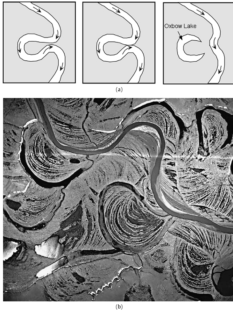
Fig. 12. (a) Cartoon showing increasing meander wavelength, terminating in meander neck cut-off and formation of an ox-bow lake. (b) Scrolled floodplains in Alaska (from Geomorphology from Space, http://geoinfo.amu.edu.pl/wpk/geos/GEO_HOME_PAGE.html ).
