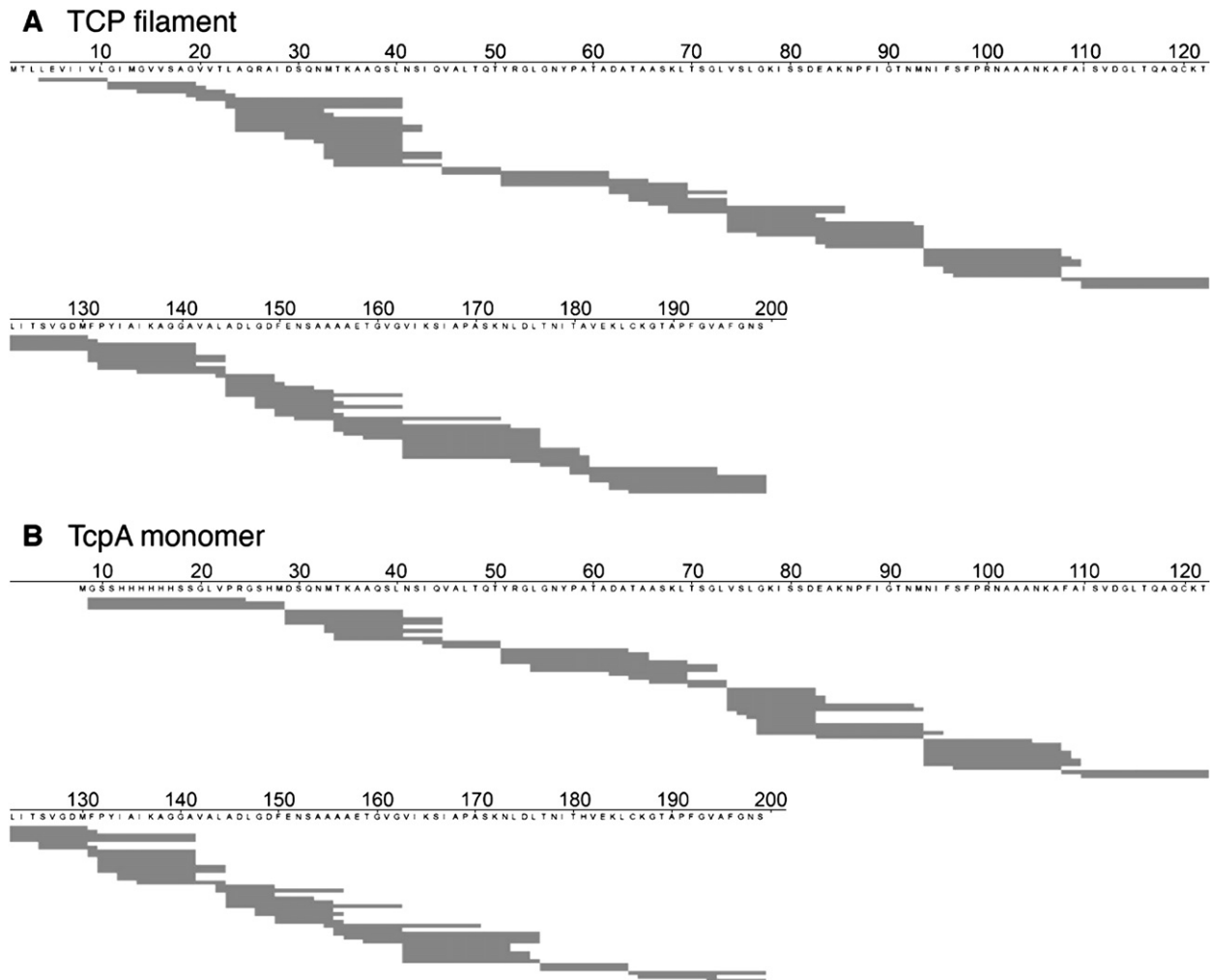
Figure 2. Overlapping Peptides Identified by Pepsin Digest and LC-MS
