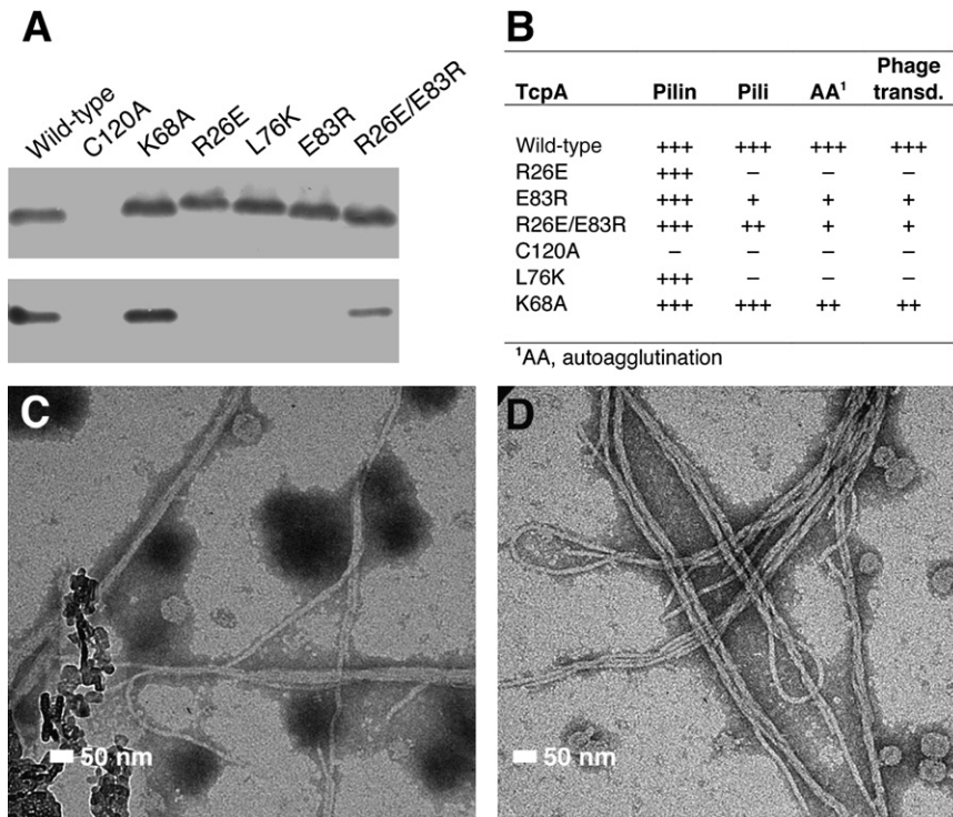
Figure 6. Analysis of Pilin Expression, Pilus Assembly, and Pilus Functions in TcpA Mutants
