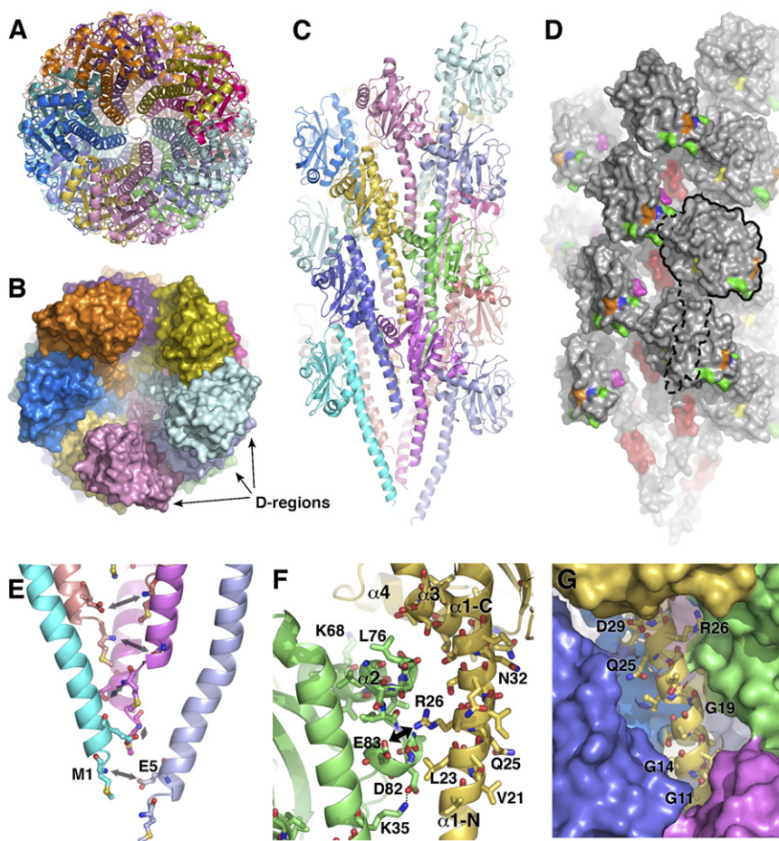
Figure 4. Refined TCP Filament Model
