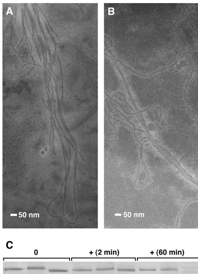
Figure 1. Comparison of Morphology and Protease Susceptibility for TCP WT and TCP H181A
