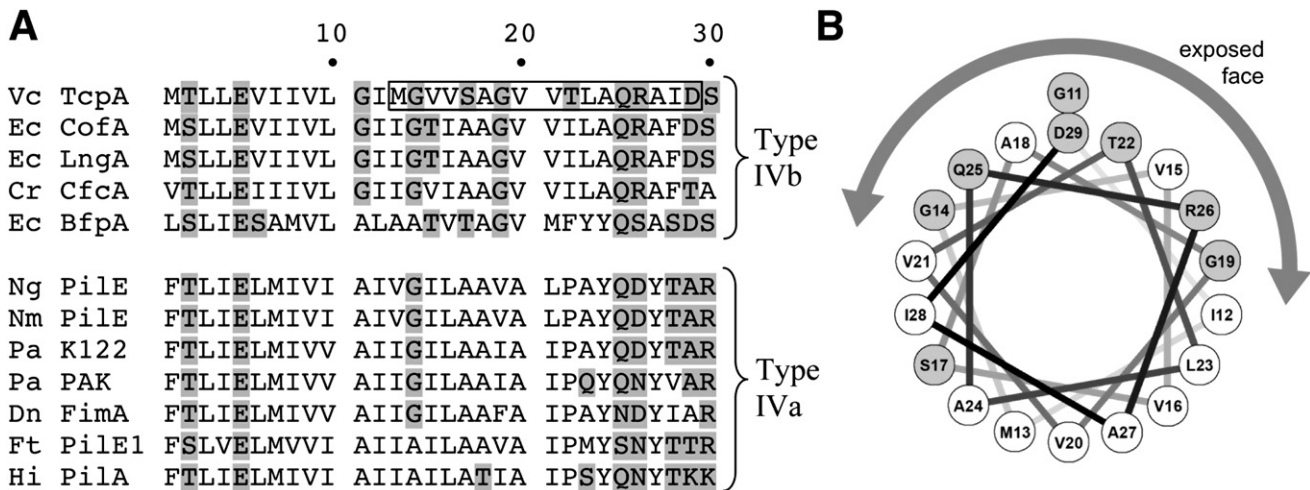
Figure 5. Amino Acid Sequence Alignments of \alpha 1-N and Helical Wheel Representation of the Amphipathic Segment
