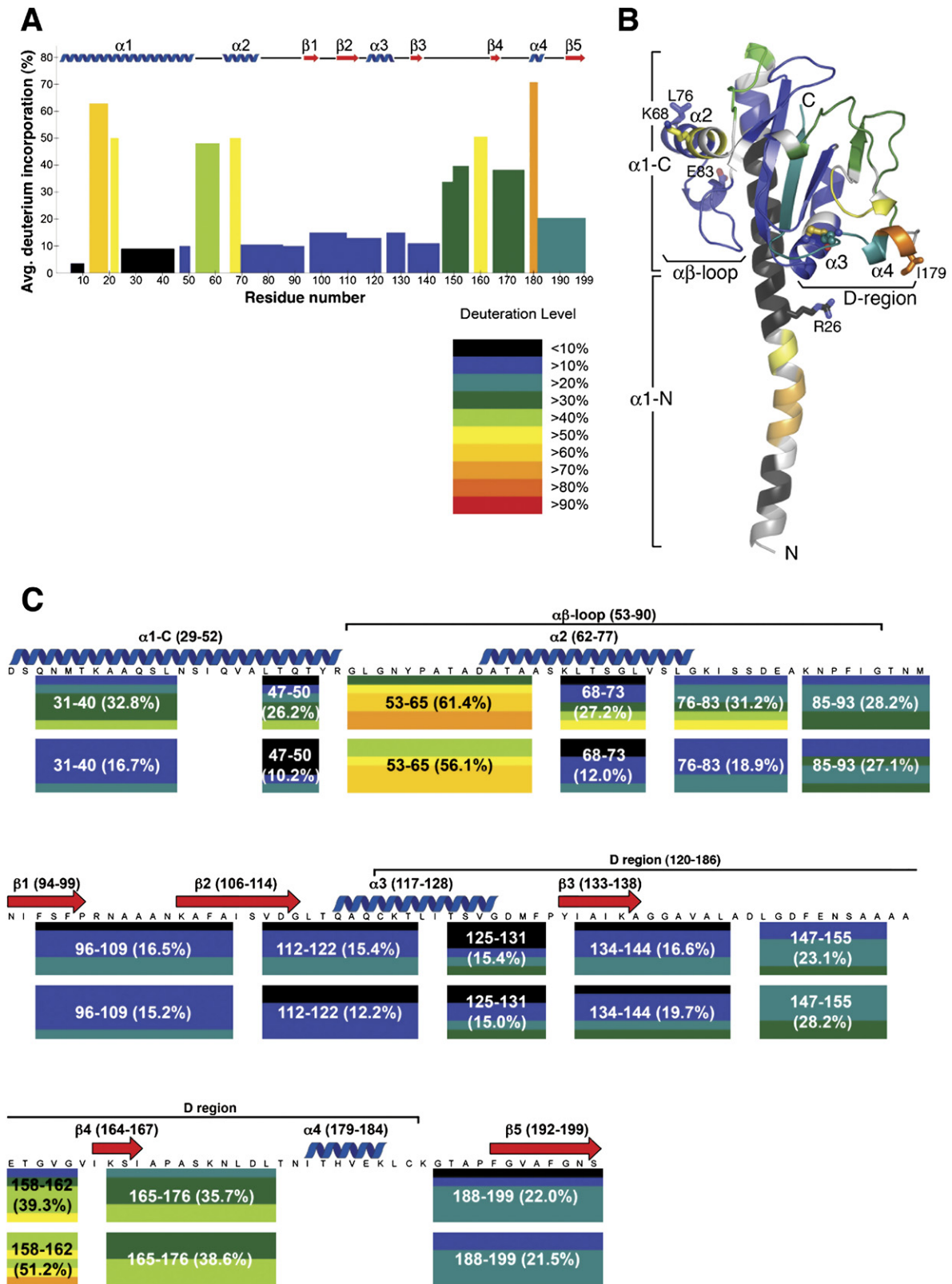
Figure 3. Deuterium Accessibility for Peptides in the TCP Filament and TcpA Monomer
