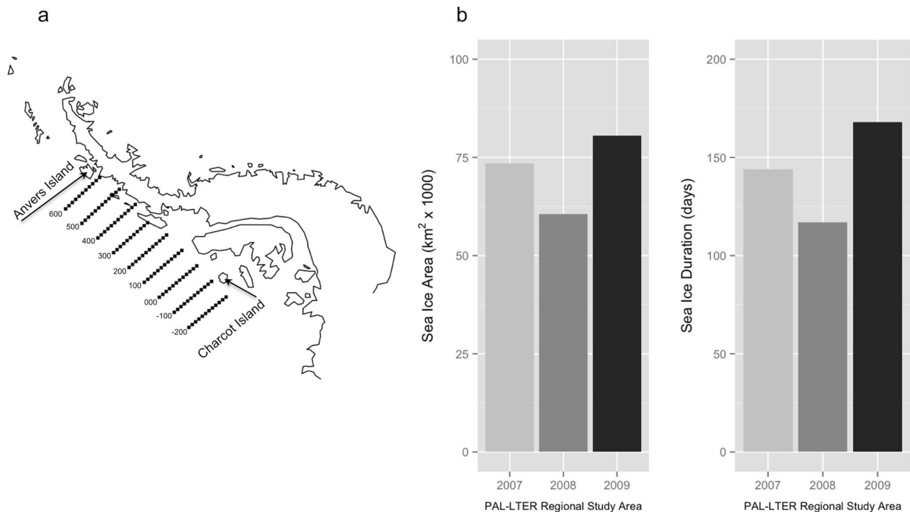
Figure 2. Palmer Station, Antarctica, Long Term Ecological Research (PAL-LTER) Program's regional study area west of the Antarctic Peninsula, extending 800 km from Anvers Island (600 line) to just south of Charcot Island (-200 line) and 220 km inshore to offshore (a). Study area grid lines encompass the entire area over which sea ice metrics were calculated. Winter average sea ice area (km 2 ) and sea ice duration (days) within the PAL-LTER regional study area for each year of the present study (b). doi:10.1371/journal.pone.0090081.g002
